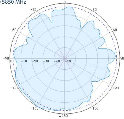
Horizontal @ 5850 MHz
