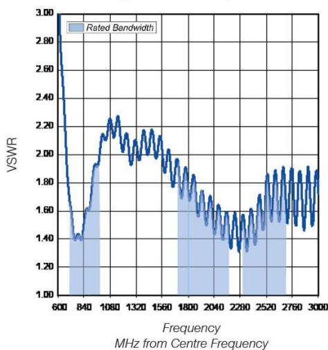
Typical VSWR Response
