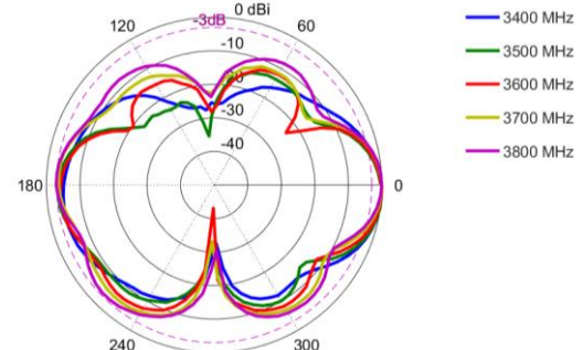
Elevation: 3400 – 3800 MHz
