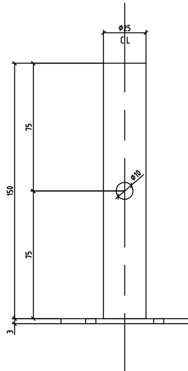
FIXED ALUMINIUM ALLOY TRIPOD FOOT
